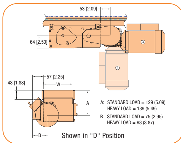
90° Gearmotor
