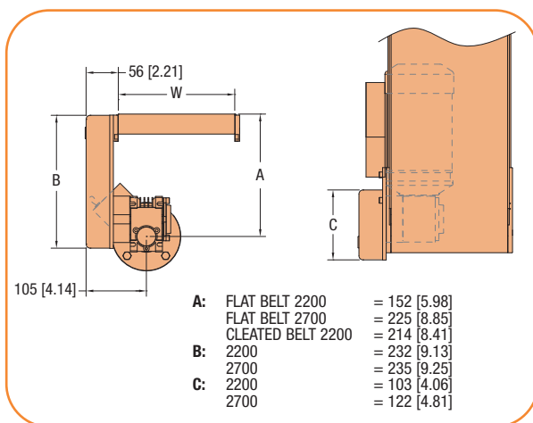
Standard Load
