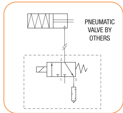
PNEUMATIC SCHEMATIC
