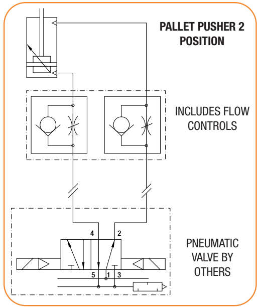
PNEUMATIC SCHEMATICS
