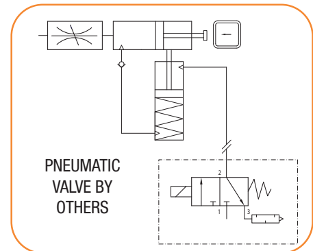
PNEUMATIC SCHEMATIC
