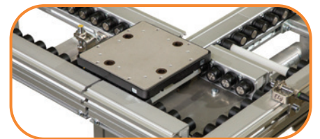
Lift & Transfer
