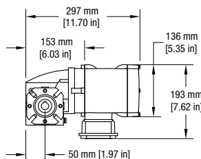
Chart 3 90 degree, Variable Speed
