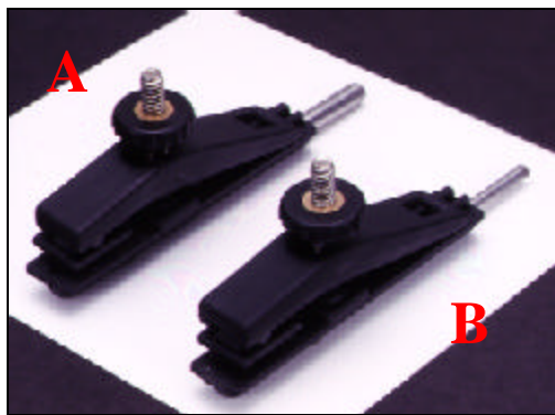
A. Profiler vise type stone holder, 1/8" shank P/N 029924 B. Profiler vise type stone holder, 3/16" shank P/N 029923
